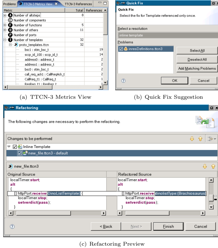
Fig. 2. TRex Screenshots
