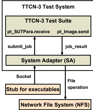
Figure 7. System Adapter
