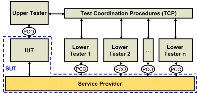
Figure 2. CTMF Multi-party test method
