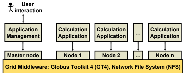
Figure 3. Application integration into the Grid environment
