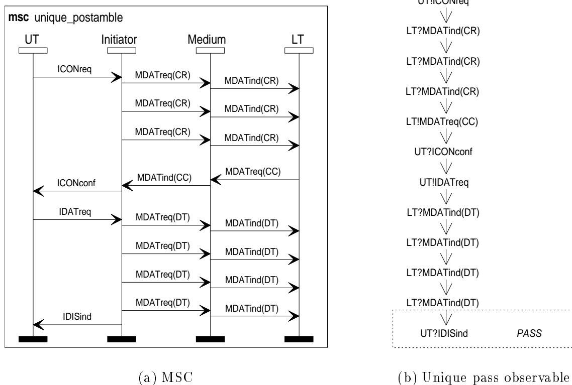
Figure 7: MSC of Figure 4 with unique postamble
